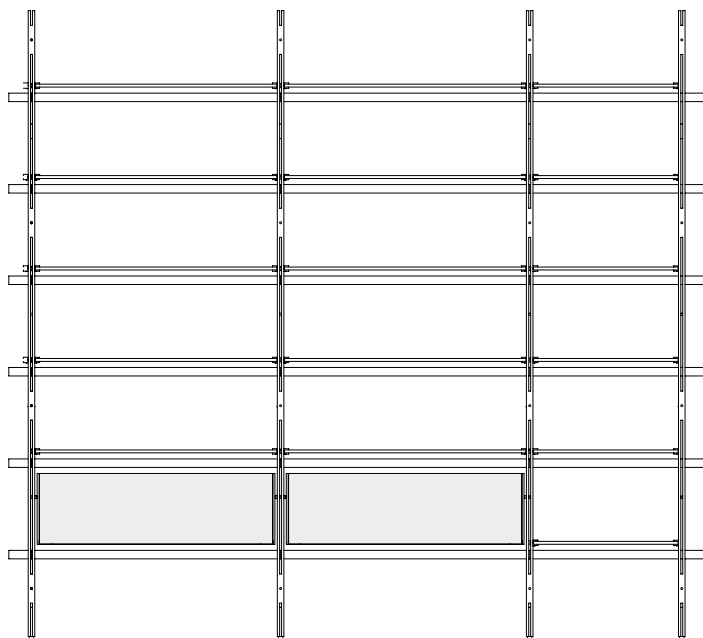
Comp. 401 286,8 x 37 x H 260 cm 4xM2 + 10xR2 + 6xR1 + 2xC3 tot. 14.820
